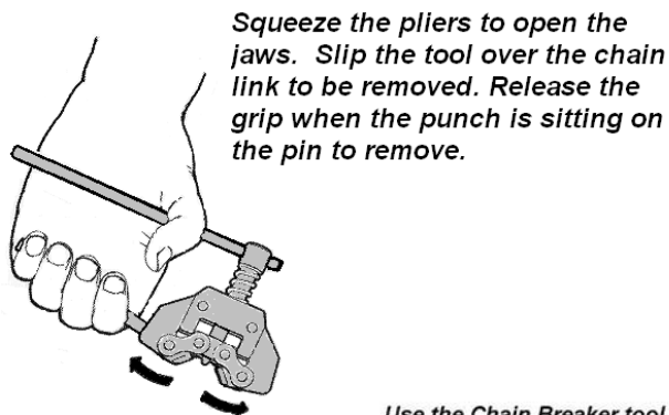
Use the Chain Breaker tool to push the pins down, forcing the link out of the chain.
