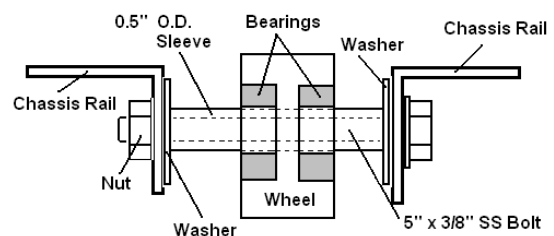
WHEEL MOUNTING IDEA
