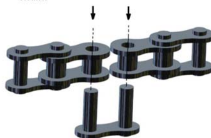
Use the Chain Breaker tool to push the pins down, forcing the link out of the chain.
